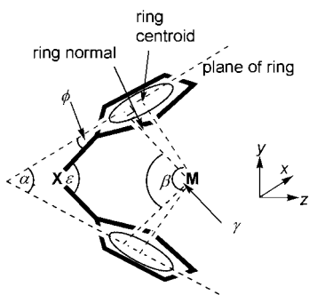
Fig. 2 Geometric parameters in an ansa -metallocene. α = angle between the ring planes; β = angle between the normals from the metal to the ring planes; γ = ring centroid–metal–ring centroid angle; ε = angle between vectors from a bridging atom X to the ipso -carbons; φ = angle between ipso -carbon vector and the ring plane.
