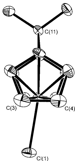
Fig. 3 Alternative view of the molecular structure of [Re{(η-C 5 H 4 )CMe 2 (η-C 5 H 4 )Cl} 1 .
