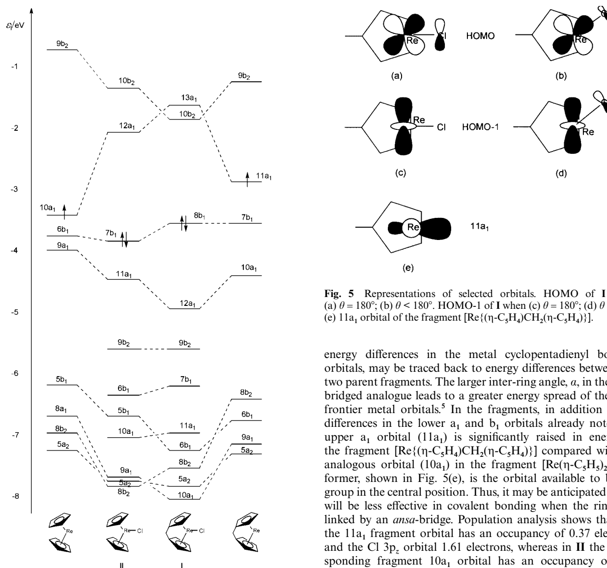
Fig. 4 MO schemes for the fragment [Re(η-C 5 H 5 ) 2 ], [Re(η-C 5 H 5 ) 2 Cl] II , [Re{(η-C 5 H 4 )CH 2 (η-C 5 H 4 )}Cl] I and the fragment [Re{(η-C 5 H 4 )CH 2 (η-C 5 H 4 )}]. Dashed lines correlate related orbitals. The levels in the schemes for I and II which are not correlated with fragment orbitals are principally chloride 3p in origin.
