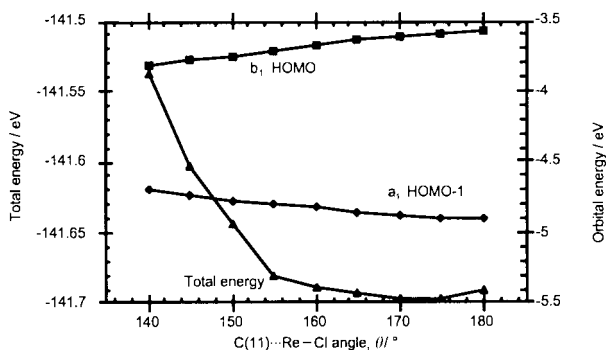
Fig. 6 Plot of the variation of the total energy, the energy of the HOMO and the HOMO-1 of [\text{Re}\{(\eta\text{-C}_5\text{H}_4)\text{CH}_2(\eta\text{-C}_5\text{H}_4)\}\text{Cl}] I , with the \text{C}(11)\cdots\text{Re}\text{-Cl} angle, \theta .
